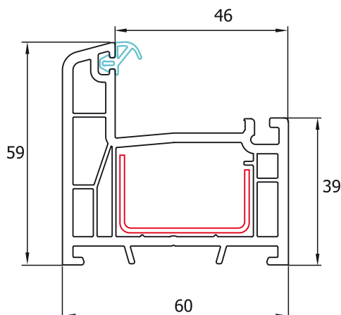
Toc mic TP4101 - standard Toc mic TP4101 - Eco Telaio piccola TP4101 - standard Telaio piccola TP4101 - Eco Kicsi Tok TP4101 - Standard Kicsi Tok TP4101 - Eco
