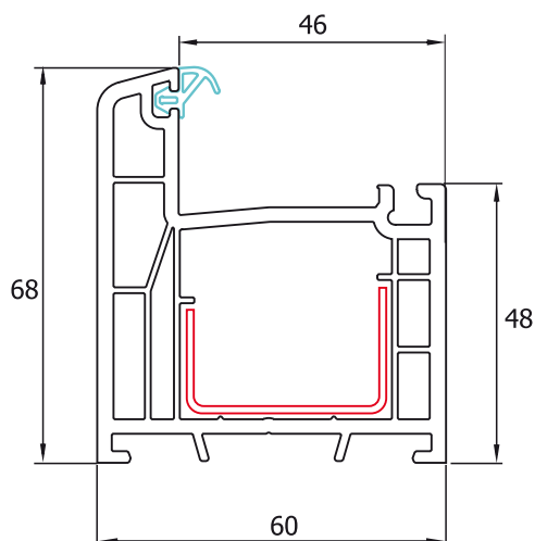
Toc mare TP4704 - standard Toc mare TP4704 - Eco Telaio grande TP4704 - standard Telaio grande TP4704 - Eco Nagy Tok TP4704 - Standard Nagy Tok TP4704 - Eco
